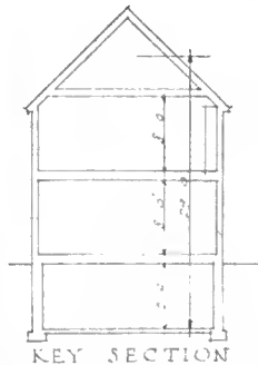
KEY SECTION
